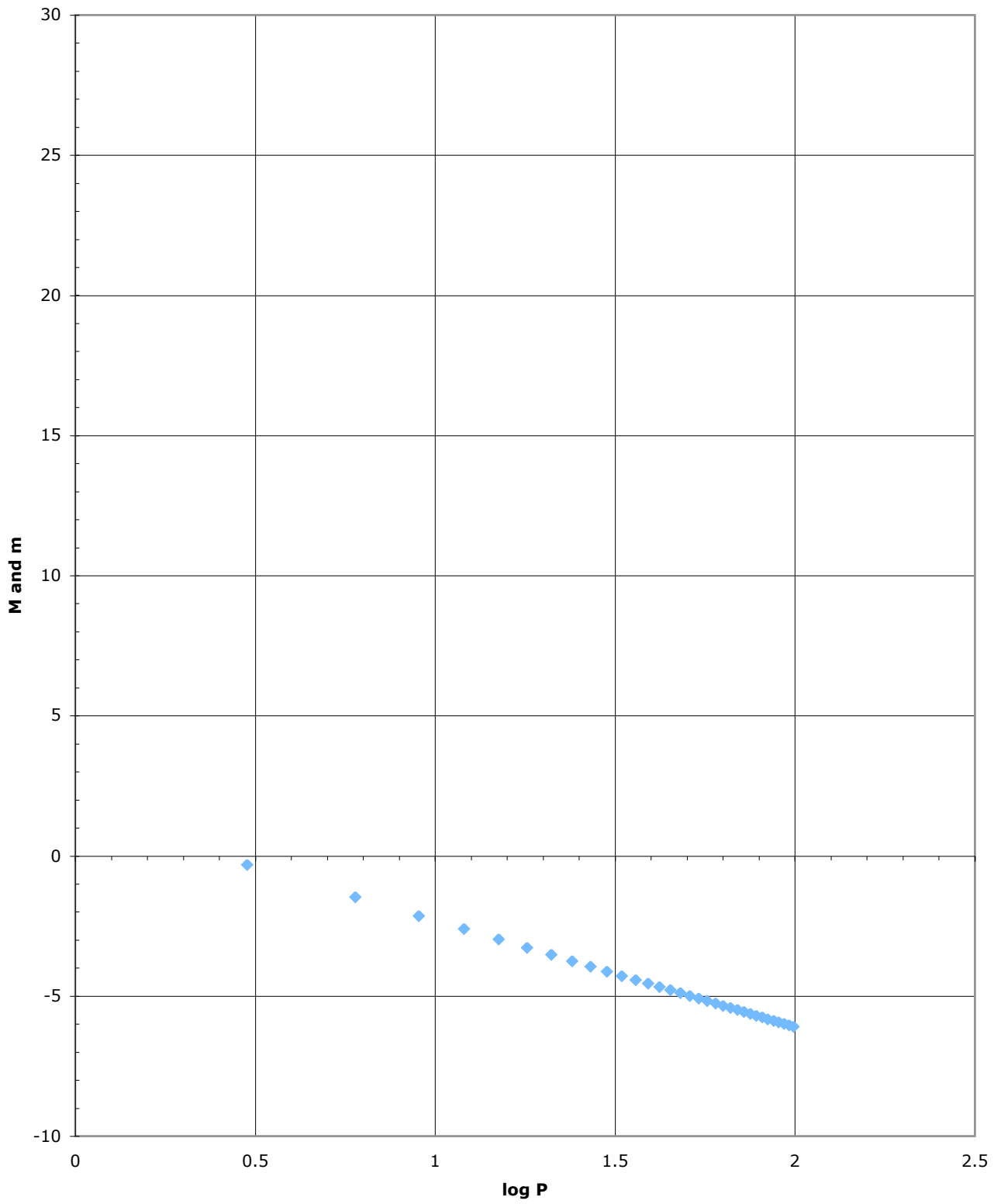
magnitude vs logP For Galaxy _____
